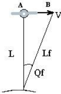
Fig.10. Ahead angle of the satellite
