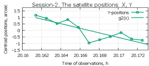
Fig. 16. Positions of the satellite along Y direction
