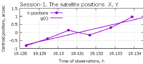
Fig. 13. Positions of the satellite along X direction
