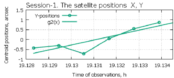
Fig. 14. Positions of the satellite along Y direction
