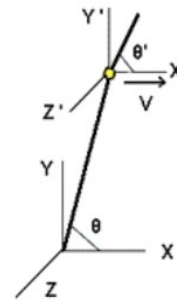
Fig.12. The laser light aberration in moving coordinate system
