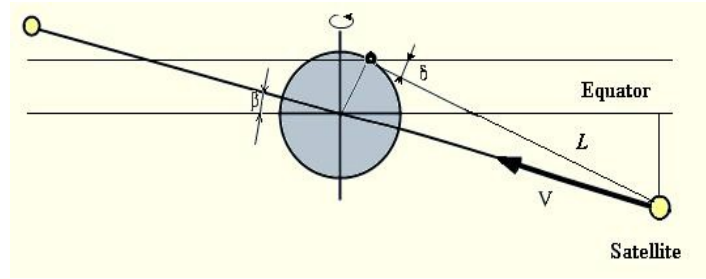
Fig. 11. Position of the satellite orbit to Equator
