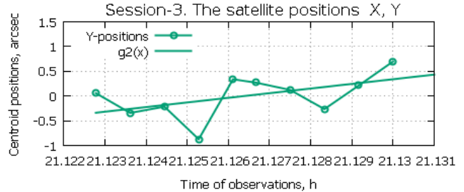
Fig. 18. Positions of the satellite along Y direction
